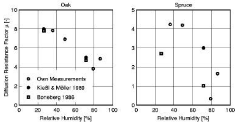
Figure 1 Measured vapour diffusion-resistance numbers in dependence on the average RH and comparison with data quoted in scientific literature.
