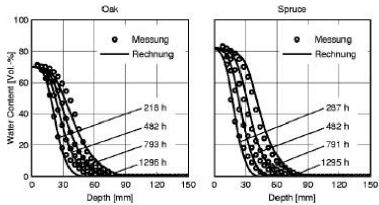
Figure 2 Measured (dots) and calculated (lines) profiles during absorption.
