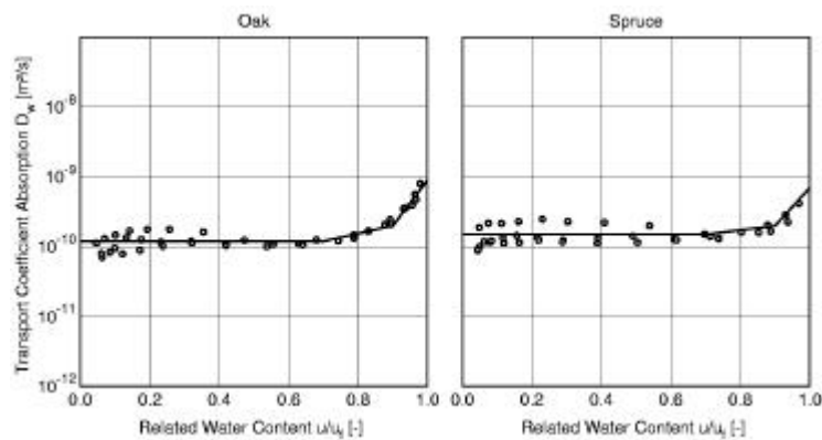
Figure 3 Capillary transport coefficients for absorption as determined from measured moisture profiles (see Fig. 2). The mean coefficients used for the calculation are represented by solid lines.
