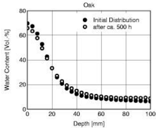
Figure 4 Moisture profiles as measured during redistribution. Even after 500 hours the initial profile has not changed considerably.
